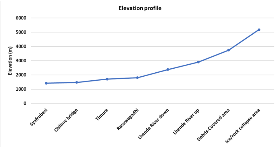
Figure 10. Elevation profile from Syafurubesi to the source area.
